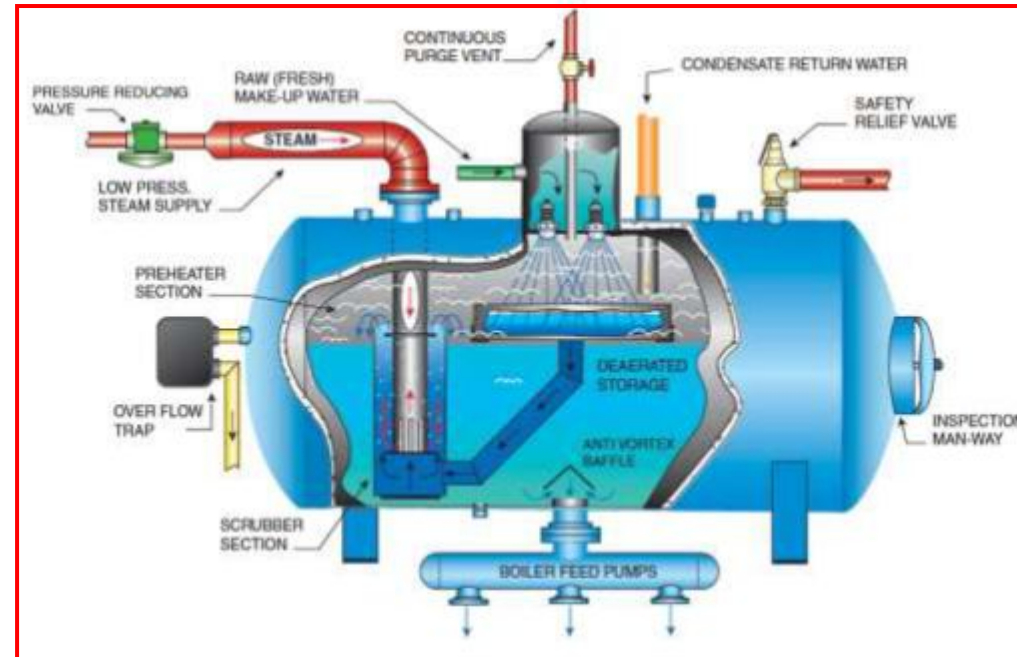
STEAM DRUM
