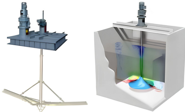
SLUDGE MIXING MACHINE
